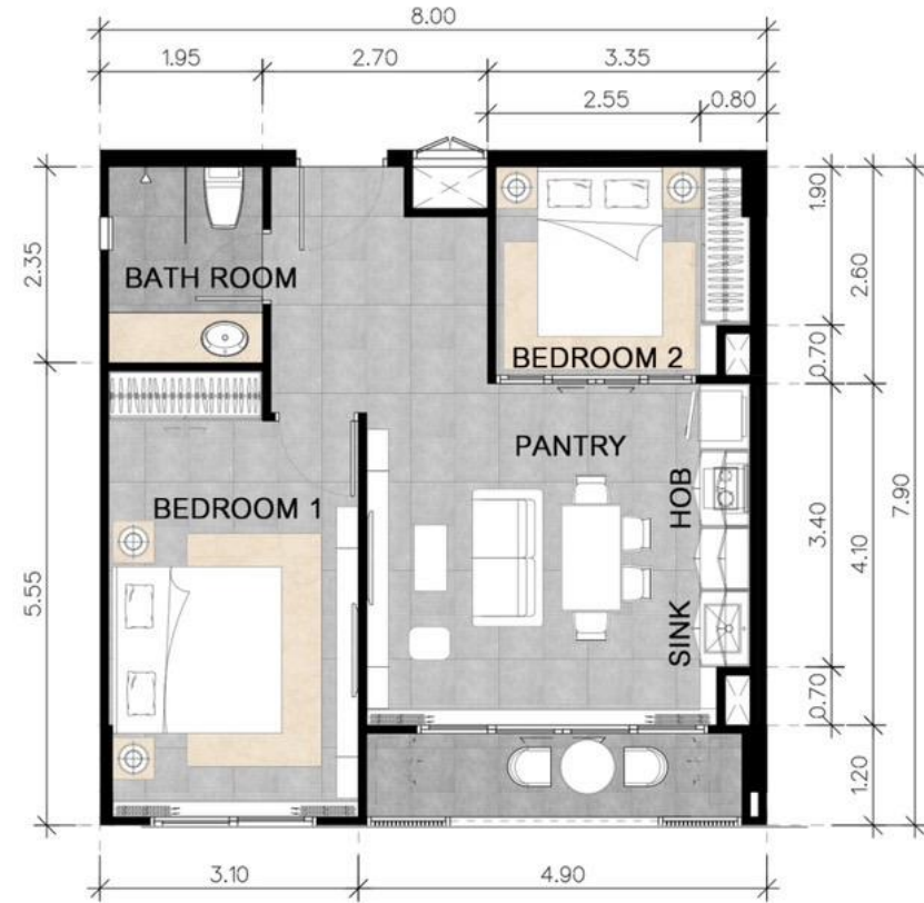
2 BEDROOM FURNITURE LAYOUT PLAN TYPE. CS TOTAL 4 UNITS AREA : 59.99 SQM.
