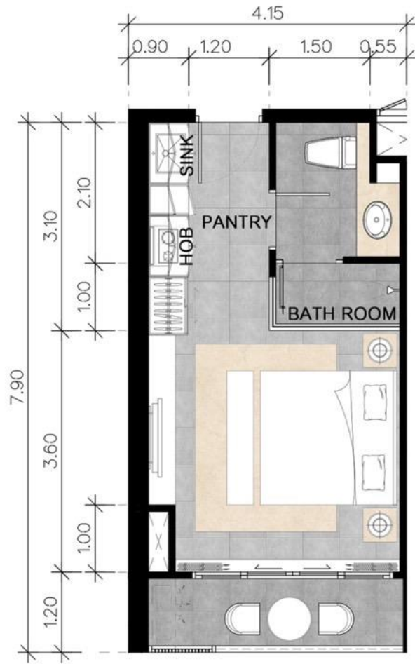
1 BEDROOM FURNITURE LAYOUT PLAN TYPE. AMS TOTAL 4 UNITS AREA : 31.54 SQM.
